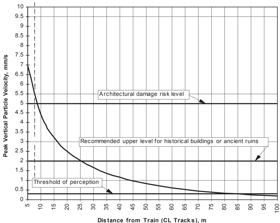
Figure 4. Maximum Train Vibration Levels vs. Distance
